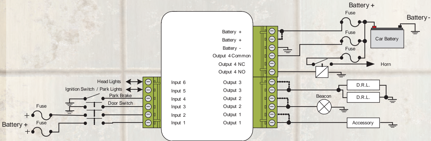
Typical Connection
